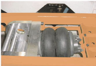
Air Bag & Pushrod Assembly
