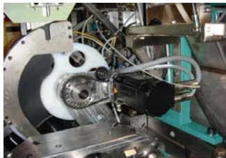
Servo Driven Rotary Cup Feed
