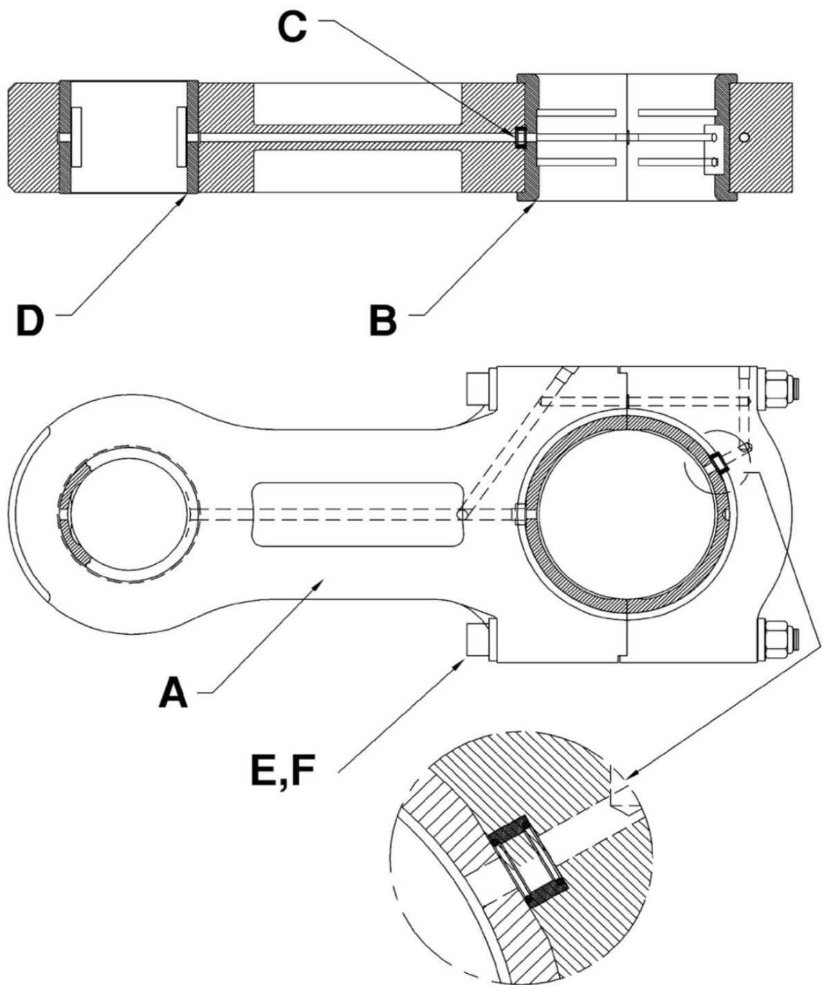
Secondary Rod Assembly (SX22i20A) Available For 19" Stroke
