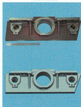
Original NO. 1998874F Slac NO. 810617 Quill
