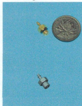
Original NO. 3413/3419(33)/C44410 Fitting PER DWG.
