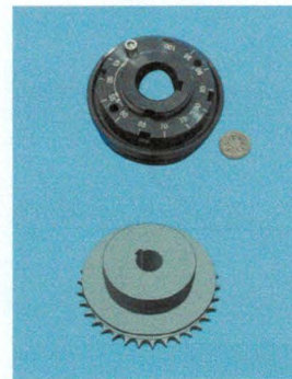
Original NO. 1299702B Slac NO. 711002 Torque Limiter
